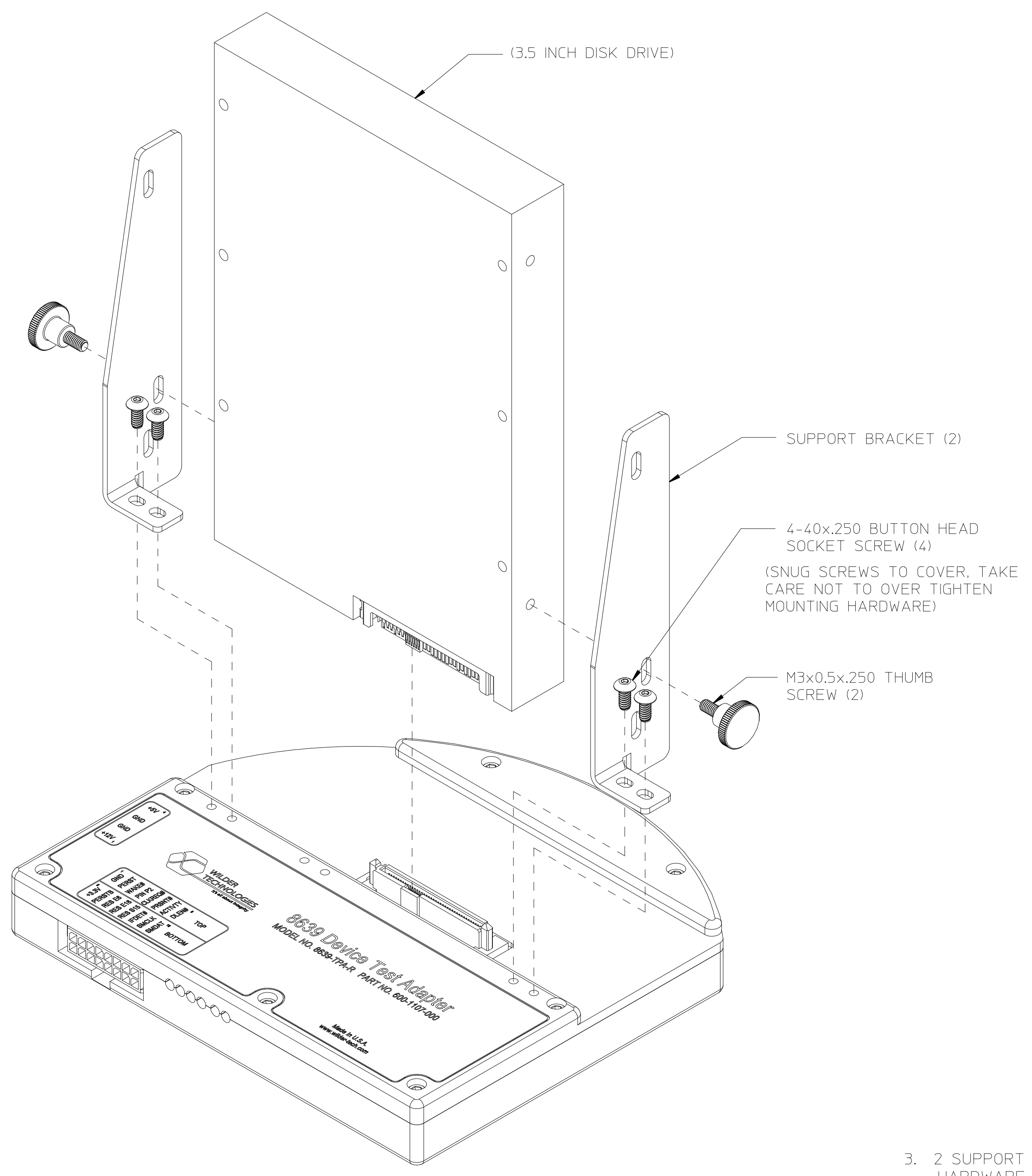
SUPPORT BRACKET INSTALLATION DETAIL FOR 3.5 INCH DISK DRIVE (CABLES REMOVED FOR CLARITY) SEE NOTE 3
