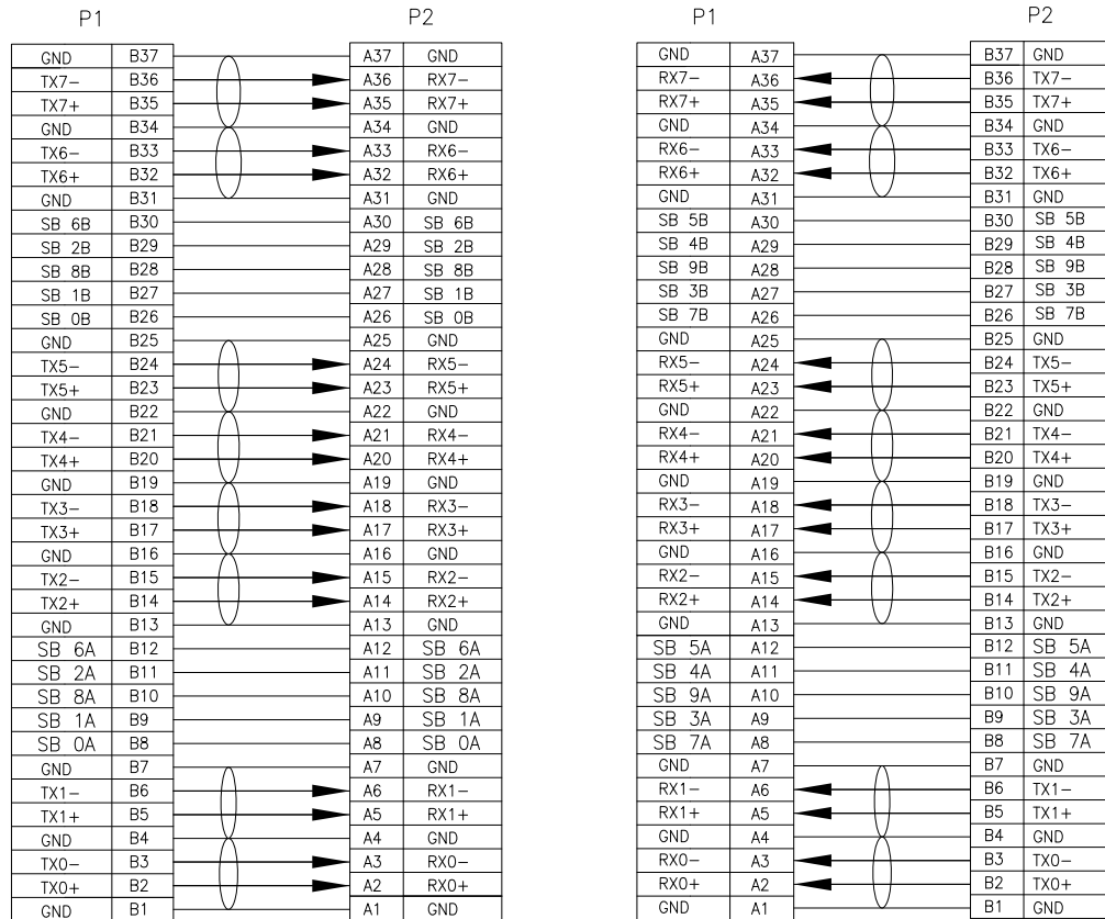
WIRE DIAGRAM
