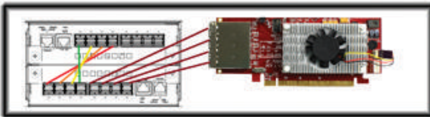
1x16 Cascaded Switches (Using SA-4444L Cables)
