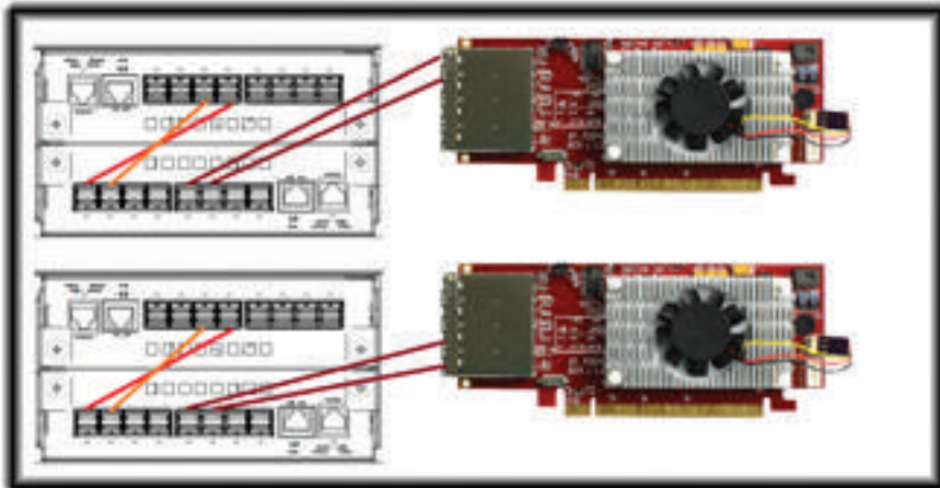
x8 Cascaded Switches (Using SA-4444L Cables)
